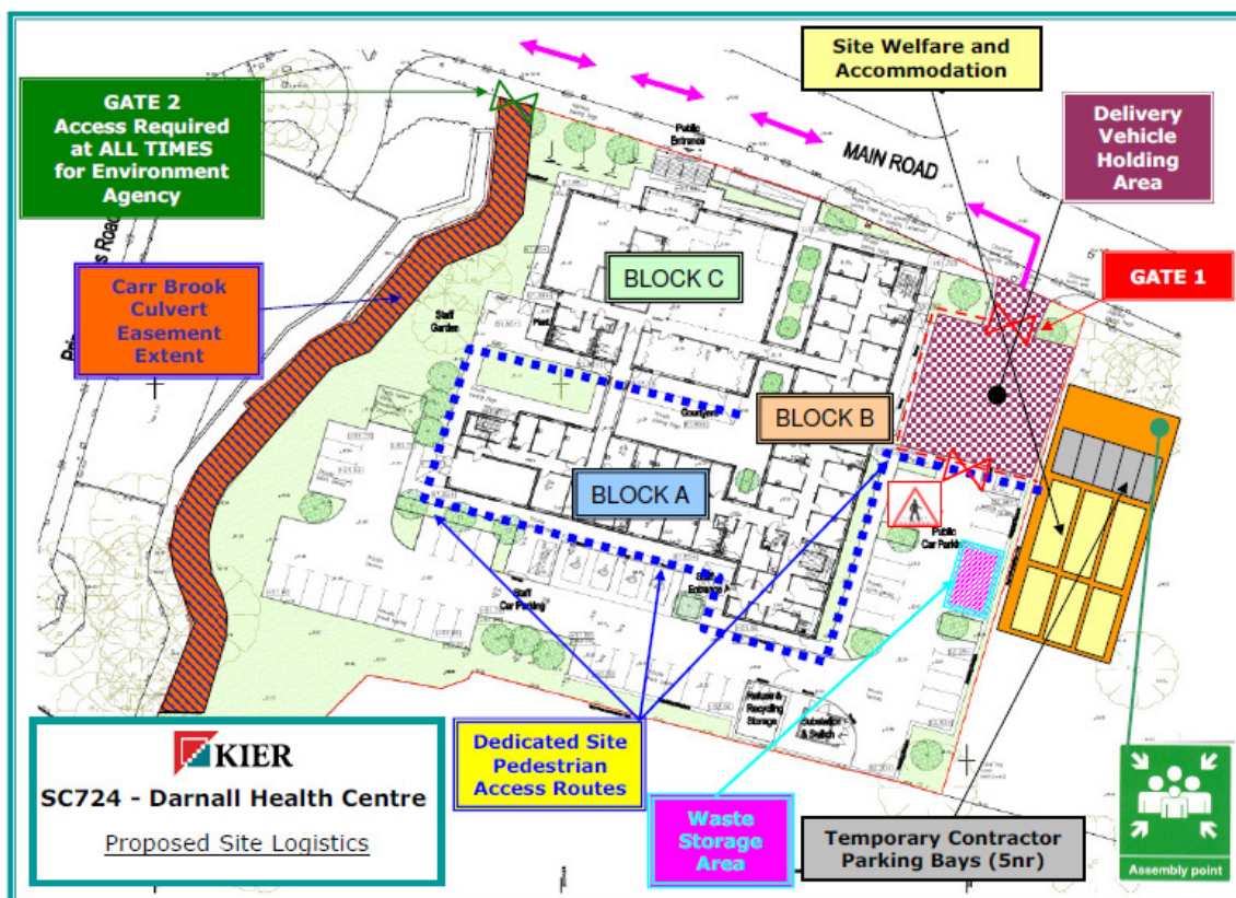
Proposed Kier Site Logistics Plan
